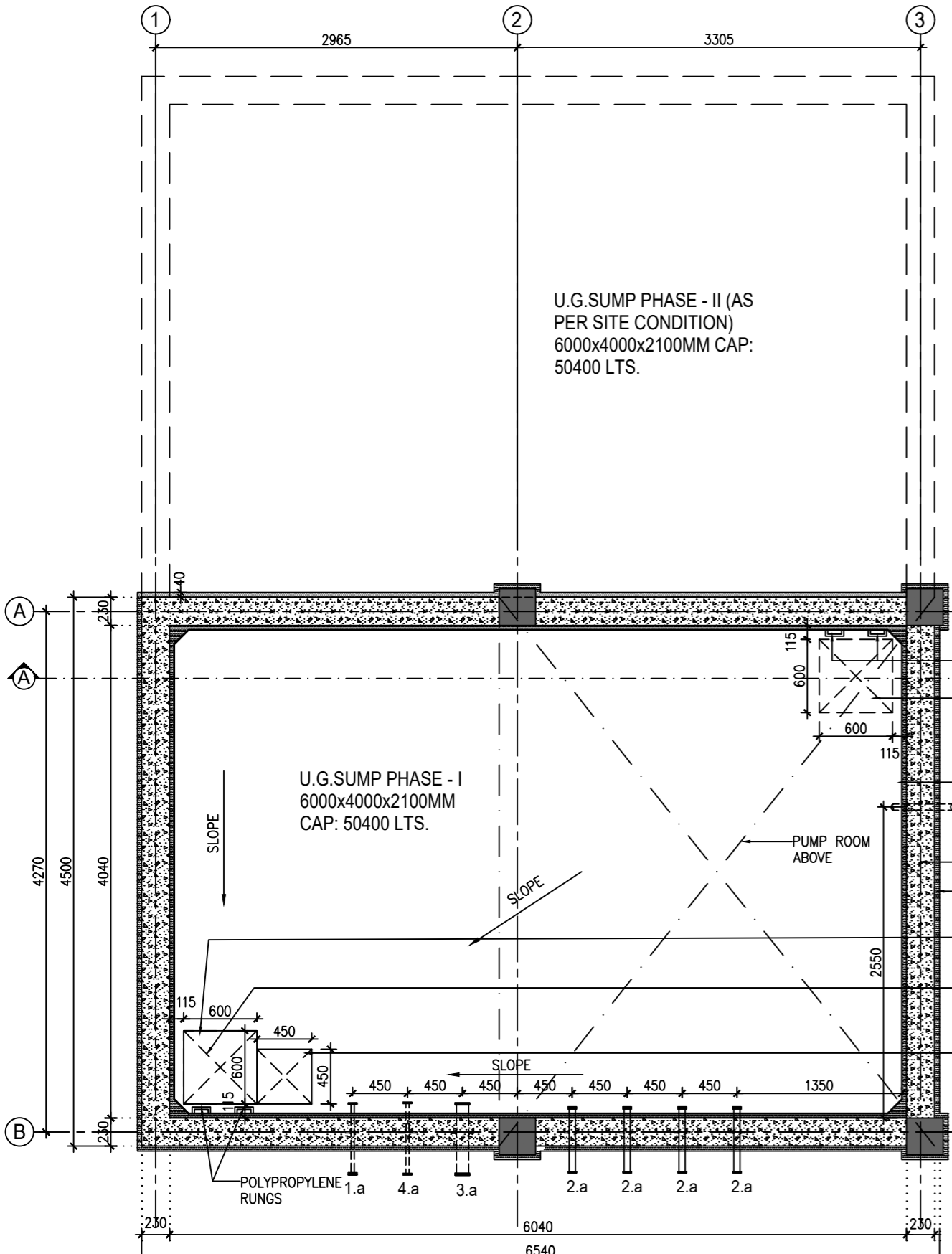
U.G. SUMP PLAN OPTION - 1
