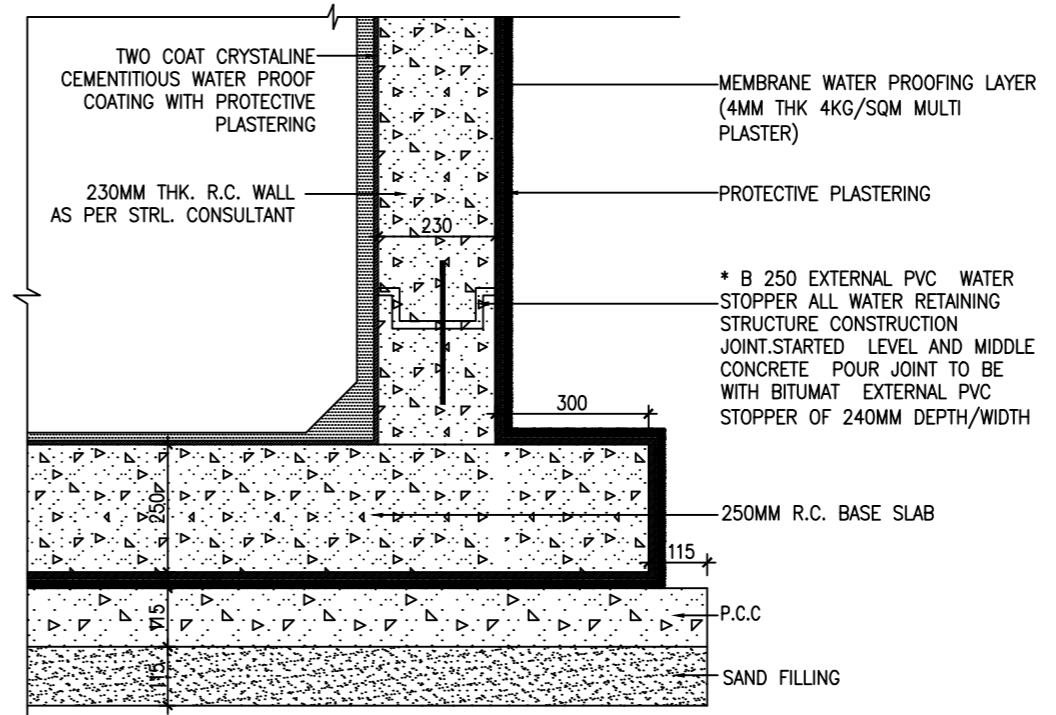
DETAIL - A
