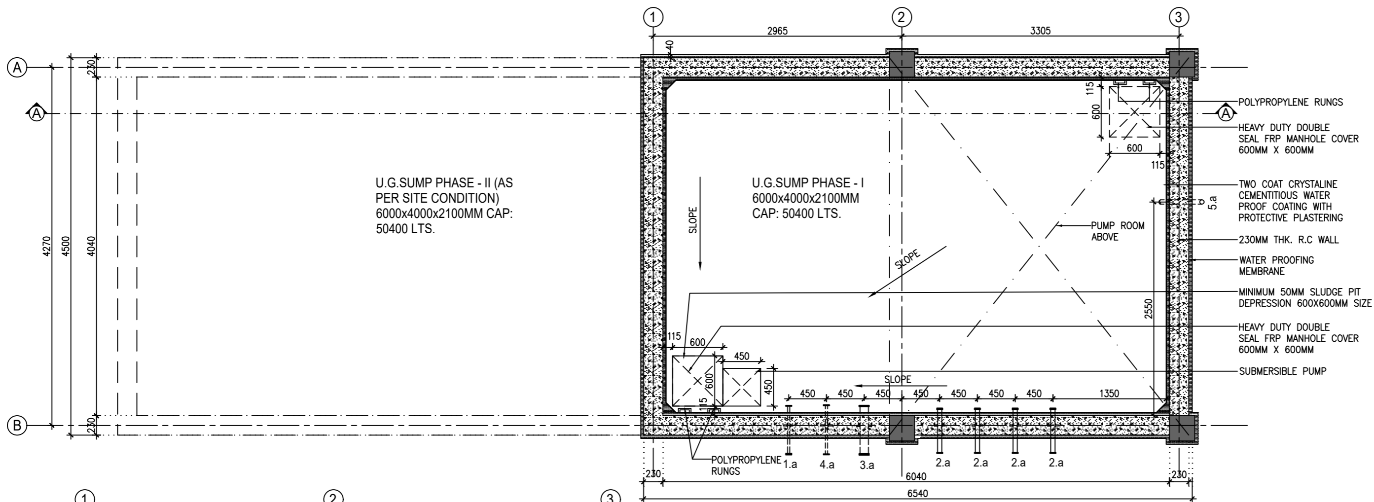
U.G. SUMP PLAN OPTION - 2
