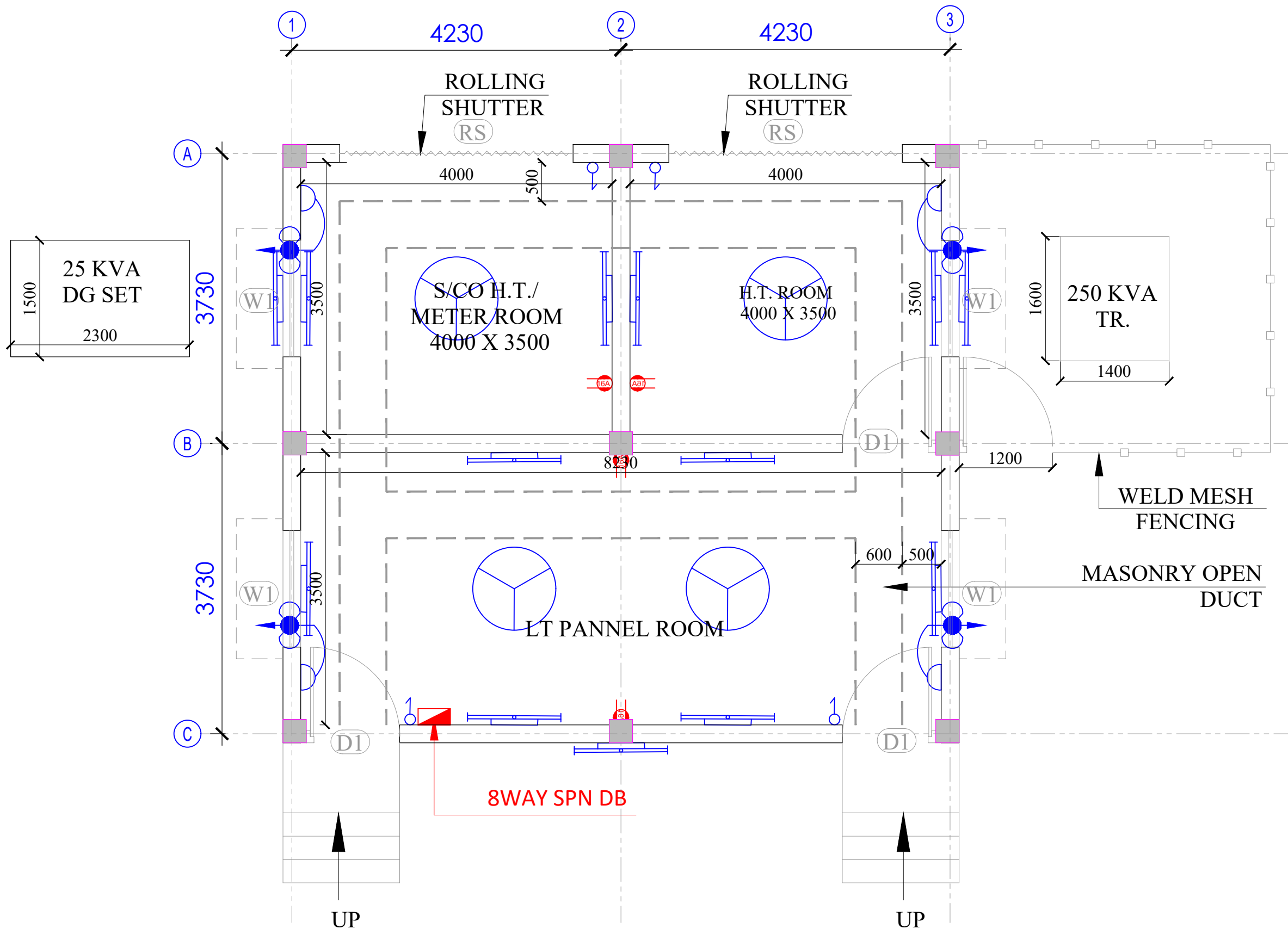
GROUND LVL. PLAN ELECTRICAL SUB STATION
