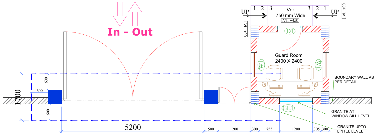
Plan At ±00 LVL.
