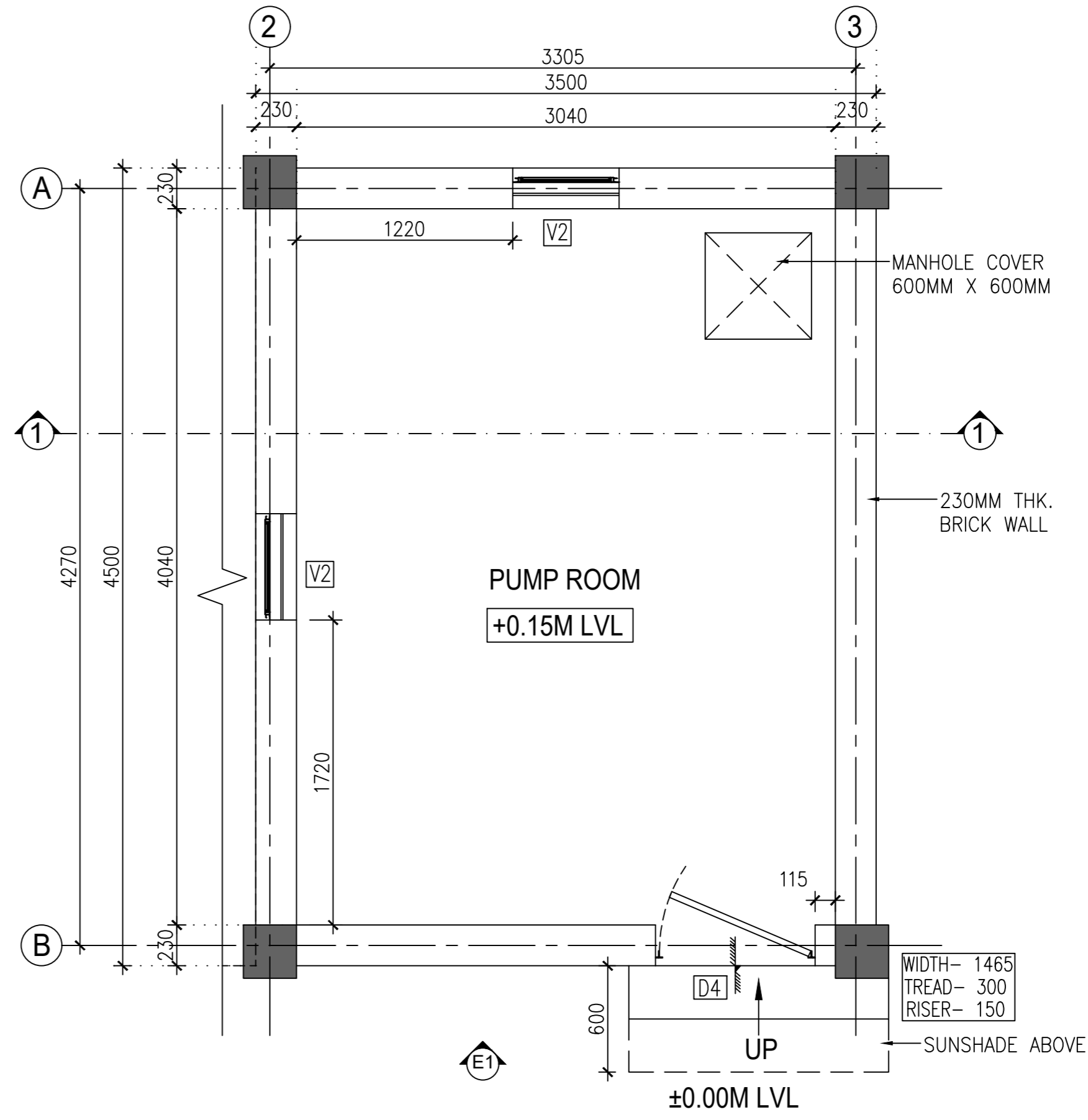
PUMP ROOM PLAN
